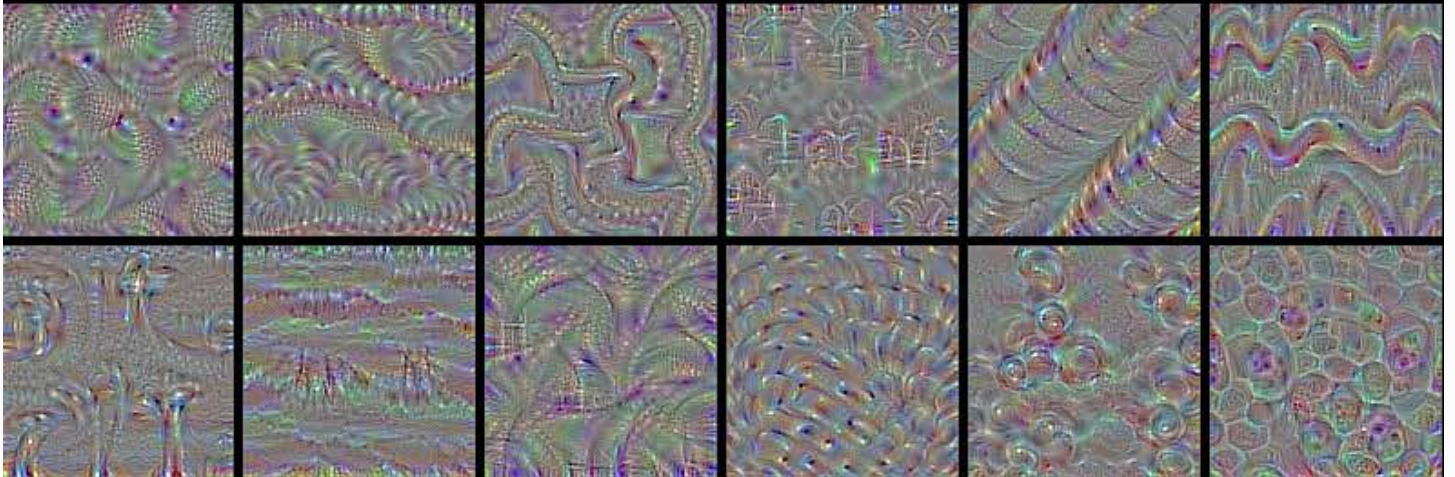
conv5_1: a few of the 512 filters
