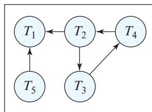
Figure 23.5 Global wait-for graph for Figure 23.4.
