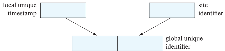
Figure 23.7 Generation of unique timestamps.
