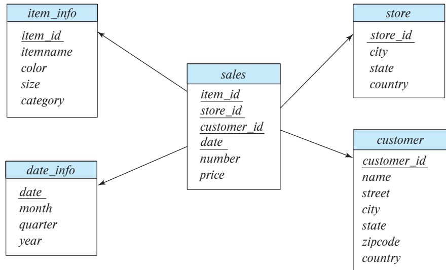
Figure 11.2 Star schema for a data warehouse.
